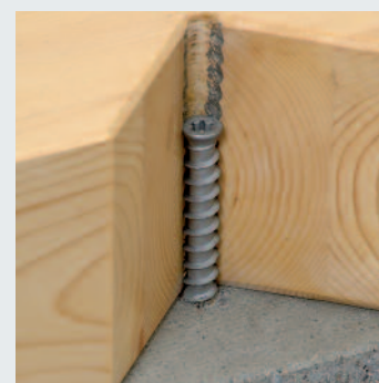
MULTI-MONTI®-TimberConnect
